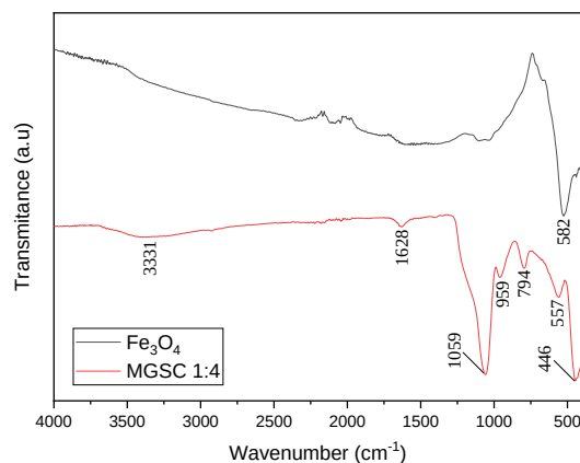
Figure 1. FTIR spectra of: \text{Fe}_3\text{O}_4 and MSGC 1:4
