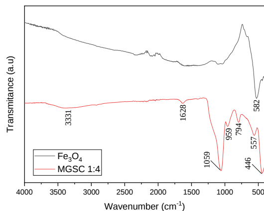
Figure 1. FTIR spectra of: Fe 3 O 4 and MSGC 1:4
